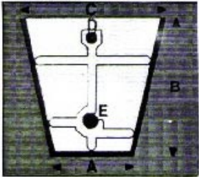
UPSIDE DOWN CASTING
