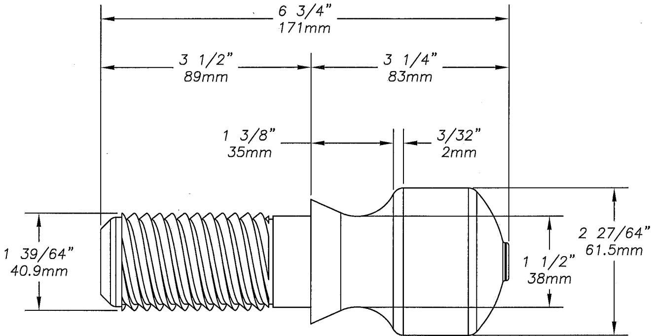
Lift Pin Dimensions
